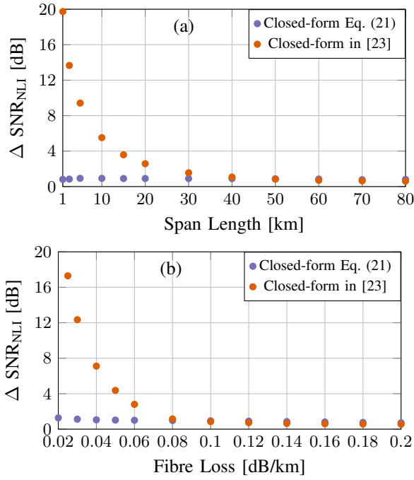
Fig. 4. Maximum per-channel SNR NLI difference ( \Delta\text{SNR}_{\text{NLI}} ) between the integral ISRS GN model and the proposed closed-form formula in Eq. (21) (purple points) for different (a) span lengths and (b) fibre losses. The \Delta\text{SNR}_{\text{NLI}} using the formula in [23] are also shown for comparison (orange points).
