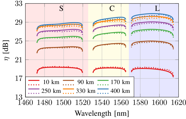
Fig. 5. Nonlinear coefficient \eta_n calculated over portions of an optical fibre link made of 5 x 80 km spans. The portions are chosen as the first 10 km of each span. The results using Eq. (21) (continuous lines) are compared with the SSFM simulations (dotted lines).
