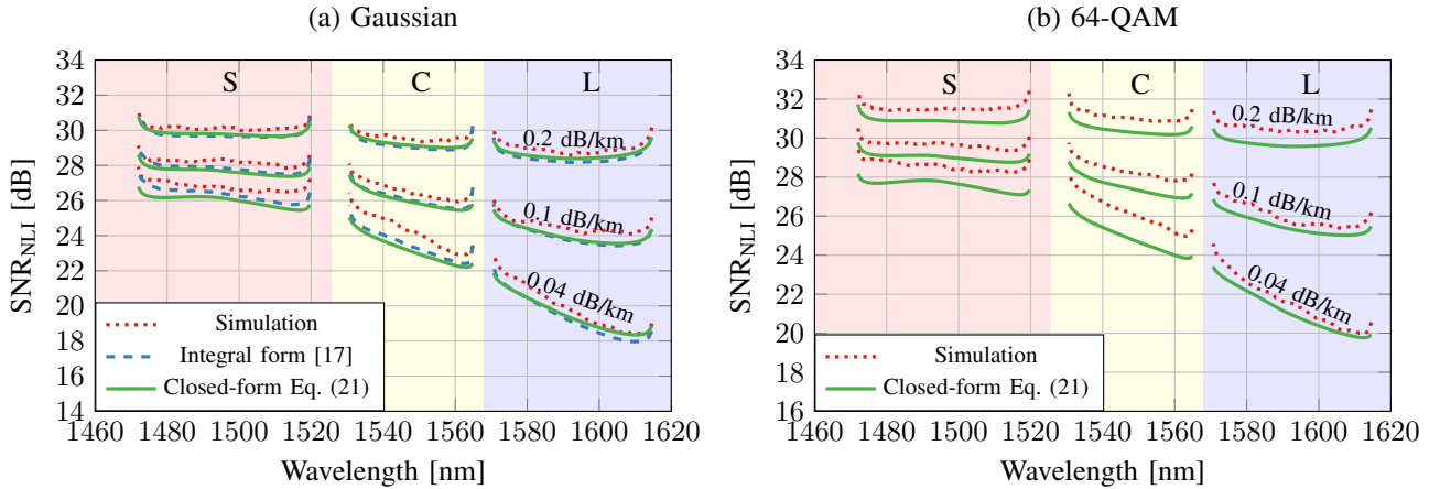
Fig. 3. Nonlinear performance for (a) Gaussian and (b) 64-QAM constellations after 5 x 80 km spans for different spectrally uniform loss profiles using the closed-form formula in Eq. (21) (green), the ISRS GN model in integral form (blue) and SSFM simulation (red).
