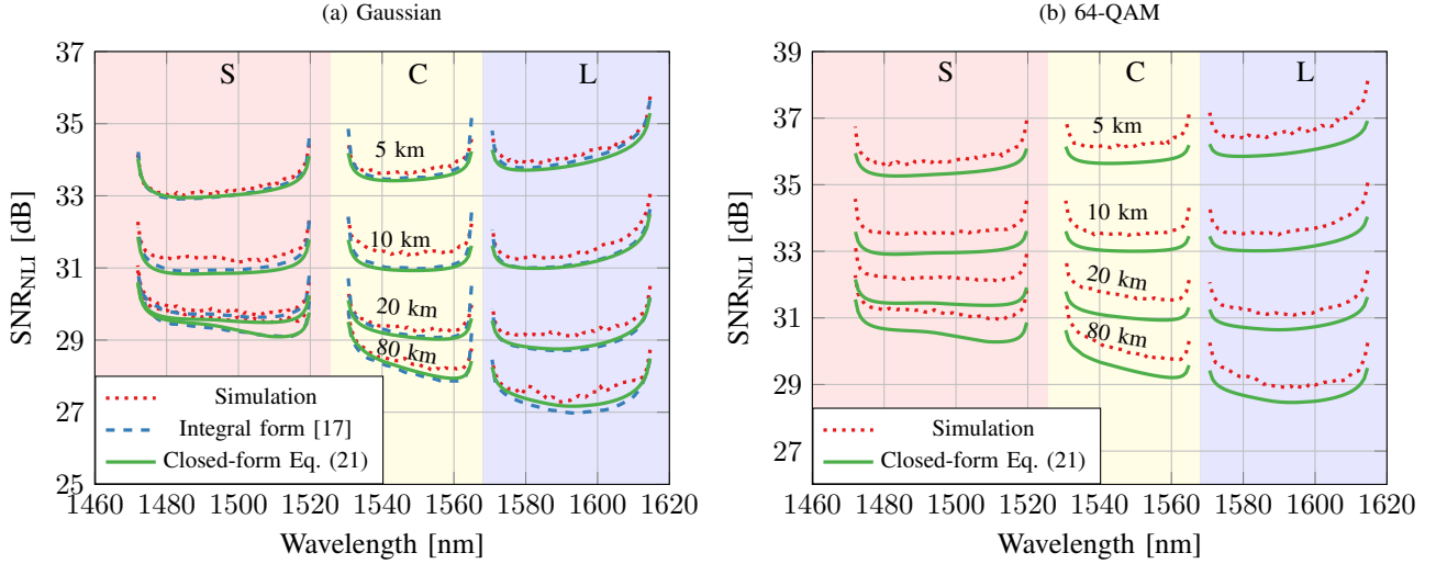
Fig. 2. Nonlinear performance for (a) Gaussian and (b) 64-QAM constellations after 5 spans for different spans lengths using the closed-form formula in Eq. (21) (green), the ISRS GN model in integral form (blue) and the SSFM simulation (red). The attenuation profile used is shown in Fig. 1.
